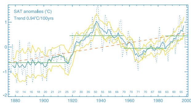
Figure 2. Composite time series of surface air temperature anomalies ( ^{\circ}\text{C} ) relative to 1961–90 for the region poleward of 62^{\circ}\text{N} . The plot displays the annual means (dashed blue), six-year running means (solid blue), 95% significance level (yellow), trend (dashed red), means for positive and negative LFO phases (horizontal green), and six-year running means using the 24 longest (century plus) records. Numbers at the bottom of the panel denote the number of stations used for averaging.
