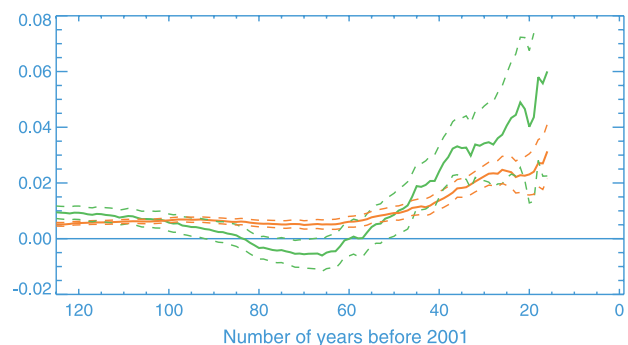
Figure 3. Arctic (green) and northern-hemispheric ([ Jones et al. , 1999], red) SAT trends ( ^{\circ}\text{C}/\text{year} ) (solid lines) and their 95% significance levels (dashed lines) computed from SAT time series, ranging from a 17 year (1985–2001) to the full record length (1875–2001), with 1 year increments.
