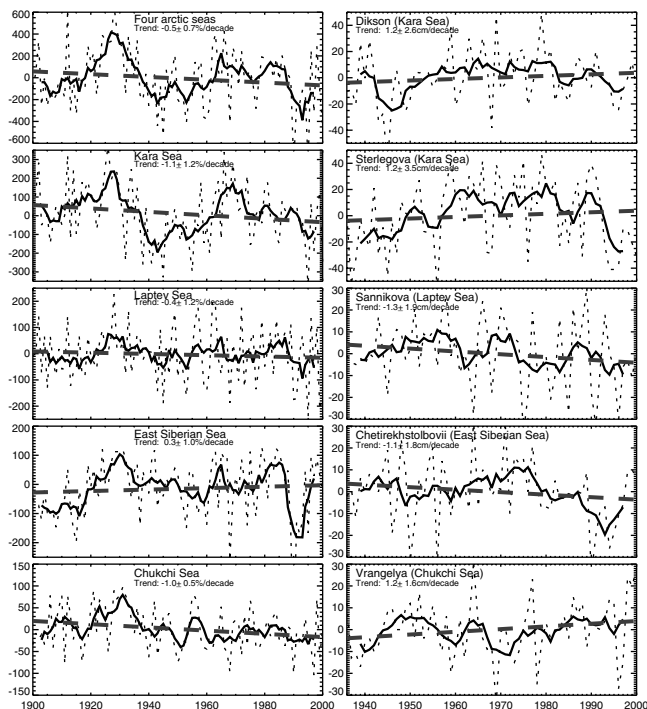
Figure 4. (Left) Time series of August ice-extent anomalies ( \times 1000 \text{ km}^2 ) in four arctic seas. (Right) Time series of annual maximum fast-ice thickness anomalies (cm) at five locations. The plot shows annual means (dotted), six-year running means (solid), and linear trends at the quoted 95% level (dashed).
