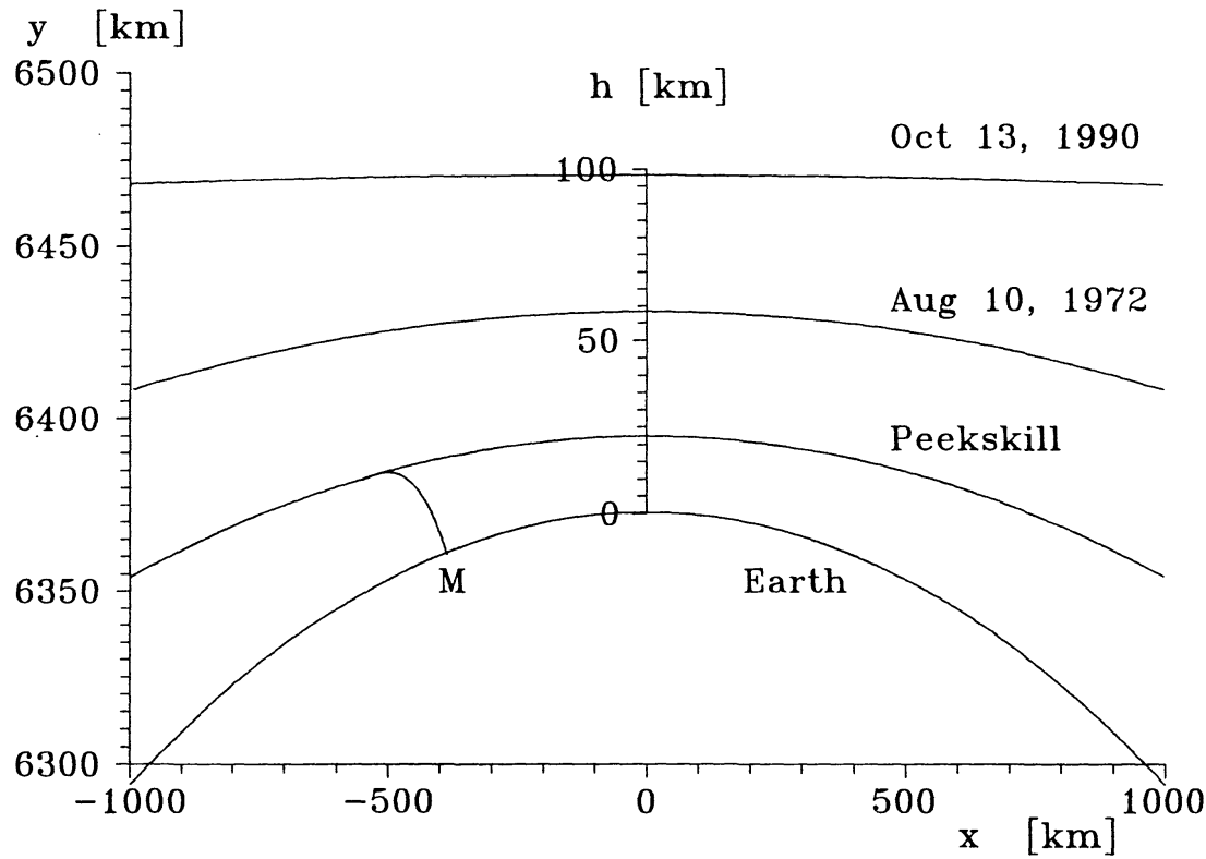
Fig. 4. Schematic representation of the Peekskill Earth-grazing trajectory in comparison the other two Earth grazing fireballs which have precise data on their trajectories available. The trajectories are put to the same apsidal line. x is the distance from the Earth center parallel the flight at perigee, y is the distance from the Earth center in the direction to perigee (very much enlarged relative to the x distances), h is the height at perigee, M is the location of the Peekskill meteorite.
